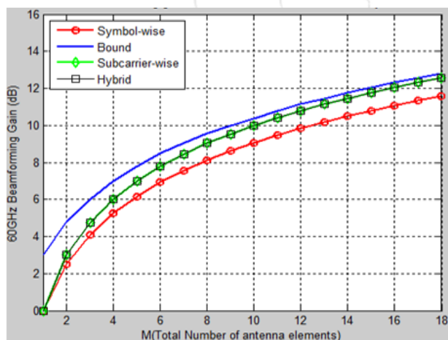
Figure 4.1: Beam forming gain vs Number of antennas in LOS
