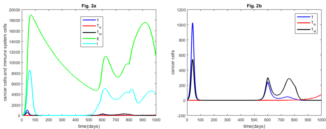
Fig. 2: Simulation results under the therapeutic approach 4.2.
