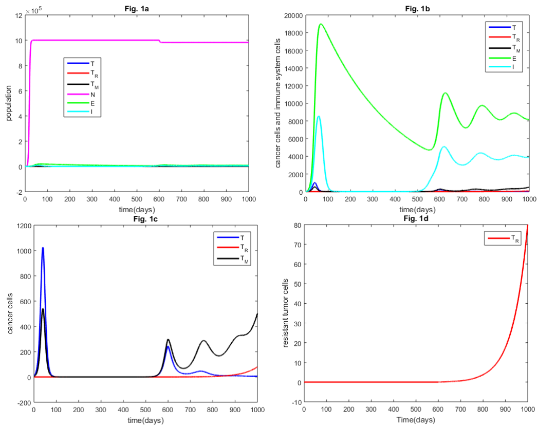
Fig. 1: Simulation results under the therapeutic approach 4.1.
