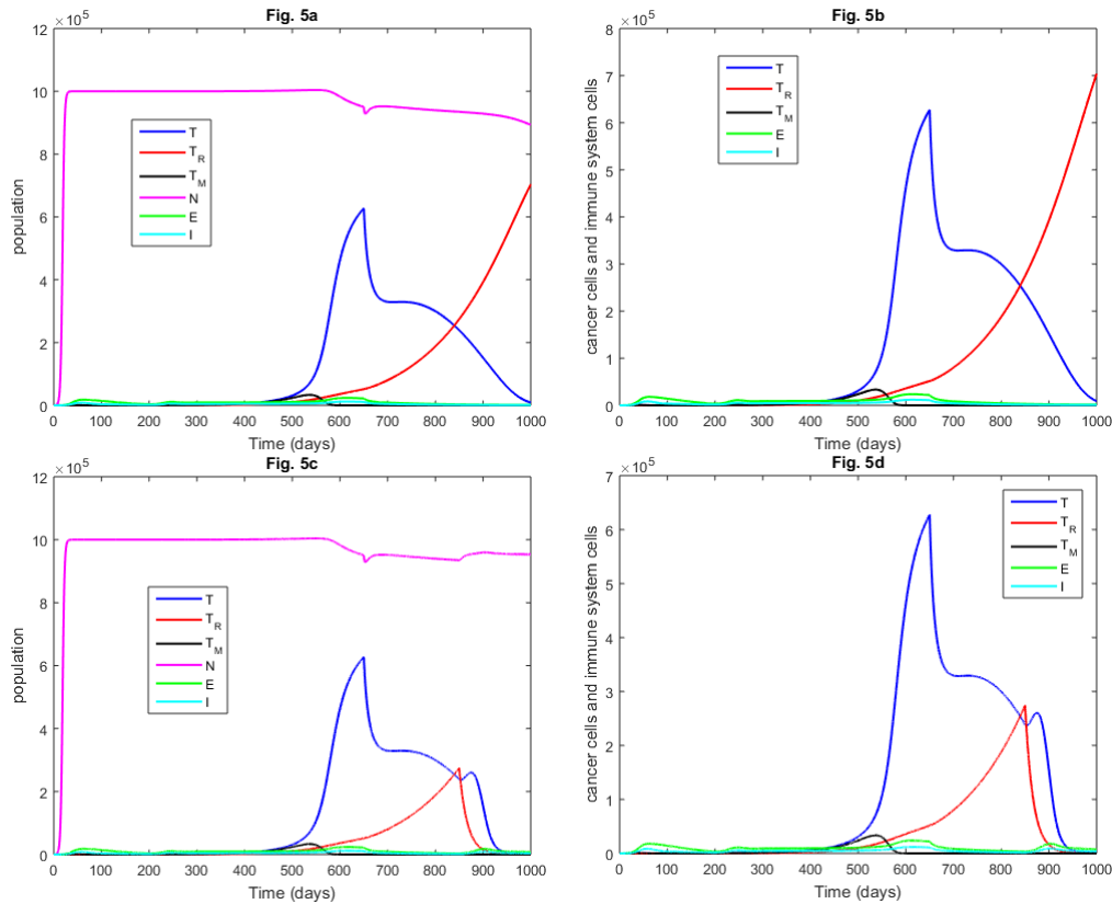
Fig. 5: Simulation results under the therapeutic approach 4.5.
