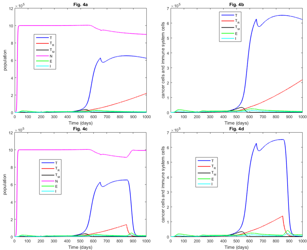
Fig. 4: Simulation results under the therapeutic approach 4.4.
