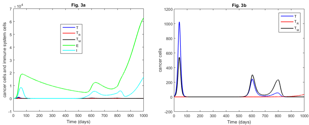
Fig. 3: Simulation results under the therapeutic approach 4.3.
