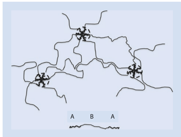
■ Fig. 7.6 Schematic depiction of a spherical morphology with a stiff polymer as the continuous phase
