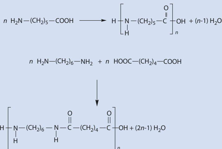
Fig. 8.29 Synthesis of (a) polyamide 6 and (b) polyamide 6,6
