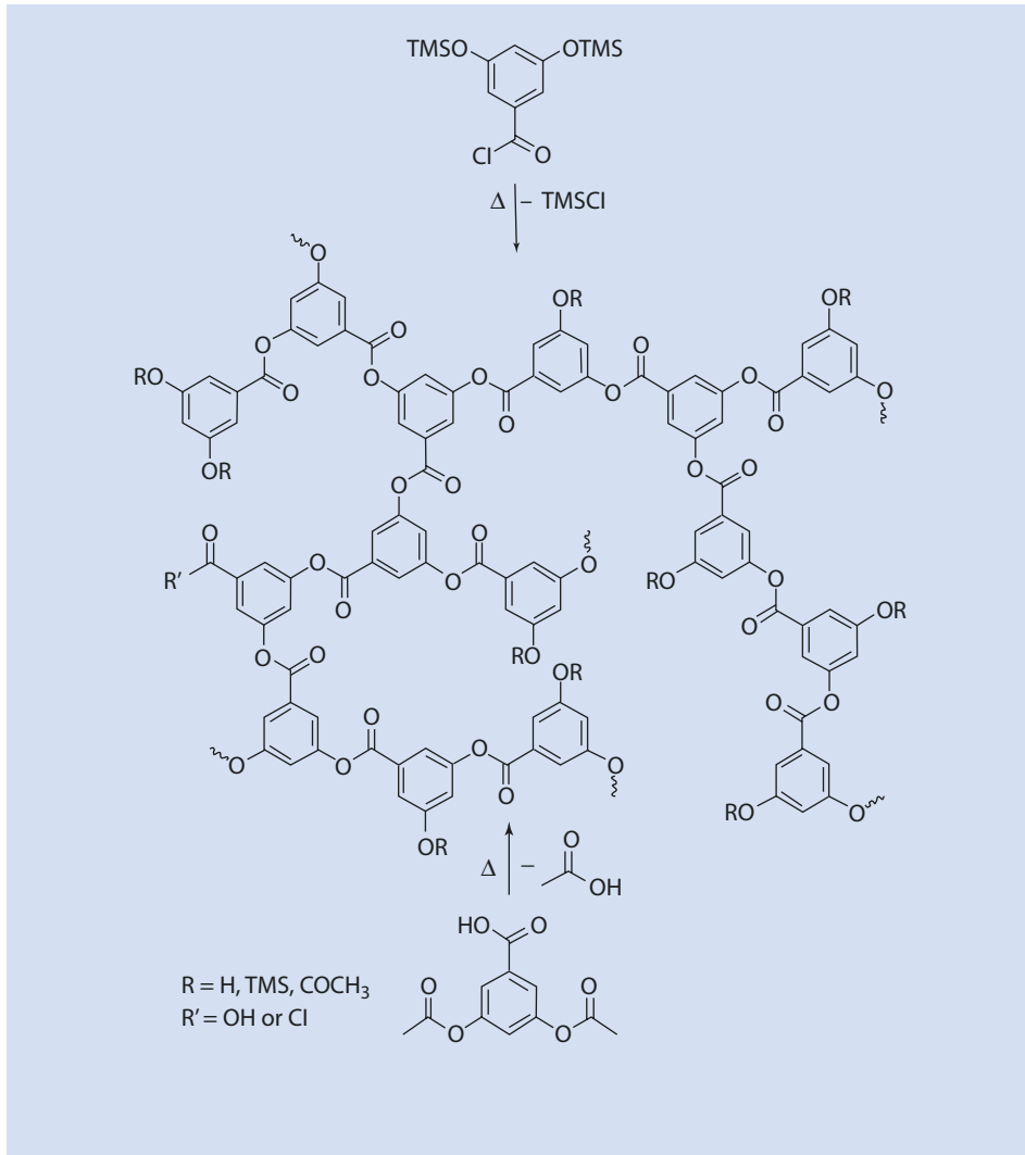
■ Fig. 8.17 Structure of a hyperbranched polyester based on two different monomers (TMS = trimethylsilyl)
