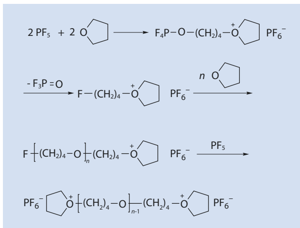
■ Fig. 12.18 CROP initiation of THF with \text{PF}_5 , chain growth in two directions
