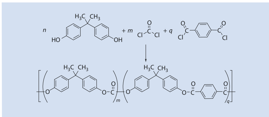
Fig. 8.28 Synthesis of a polyestercarbonate ( m + q = n )
