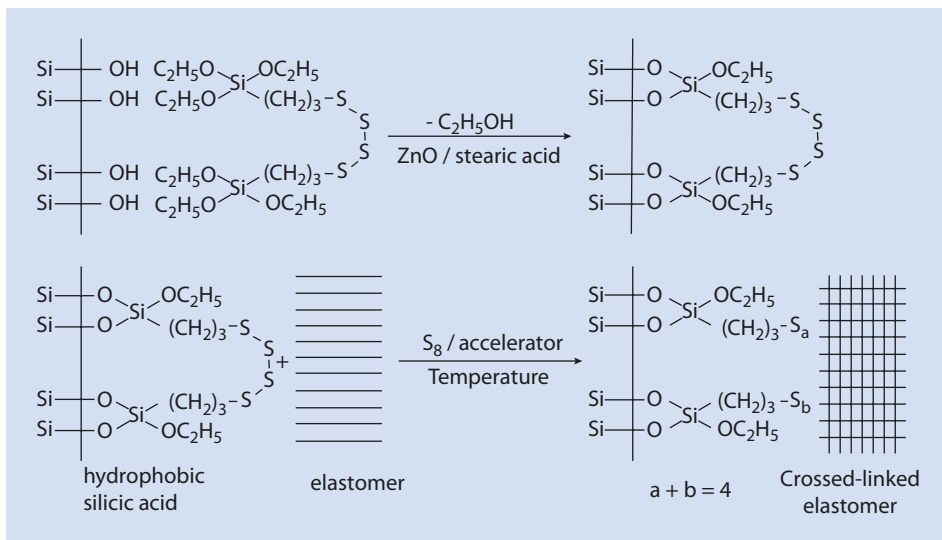
■ Fig. 7.26 Si69 ° as a coupling agent between silica and a rubber matrix
