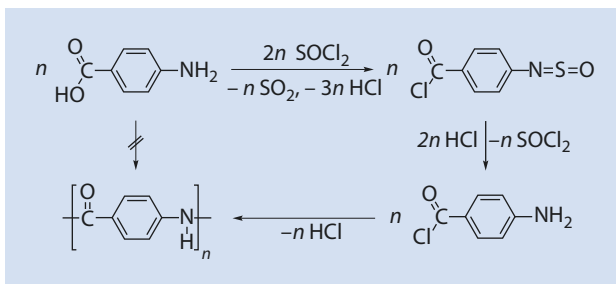
■ Fig. 8.34 Formation of an aromatic polyamide from 4-aminobenzoic acid indirectly via the Schotten–Baumann reaction
