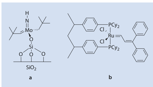
Fig. 11.29 The immobilization of well defined metathesis catalysts. (a) Schrock-type on \text{SiO}_2 . (b) Grubbs-type on polystyrene
