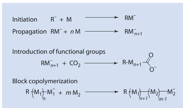
■ Fig. 10.48 Reactions of anionic species with monomer and terminating reagents, here: \text{CO}_2 , M , M_1 , M_2 monomers
