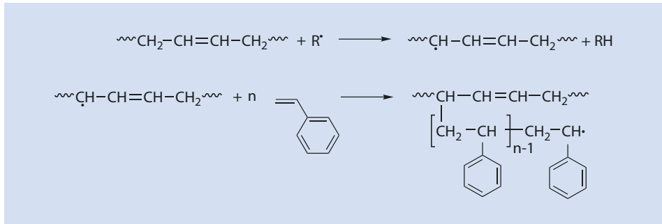
Fig. 14.13 Styrene-butadiene graft copolymers resulting from chain transfer to polybutadiene. The reaction between polystyrene and polybutadiene radicals also leads to graft copolymers. \text{R}^\cdot can be an initiator or a polystyrene radical
