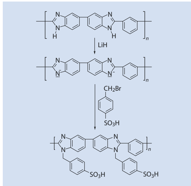
Fig. 22.23 Sulfonation of PBI (Glipta et al. 1997)
