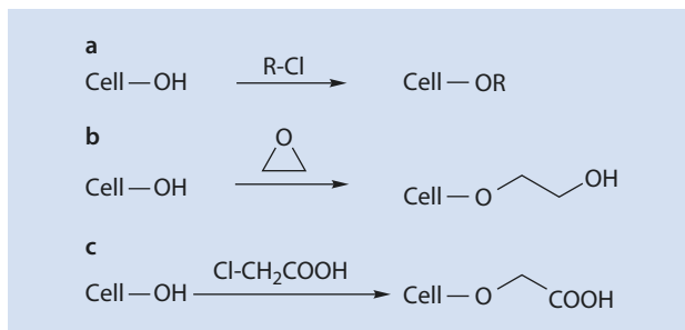
■ Fig. 15.9 Reaction of cellulose to (a) cellulose ethers, (b) hydroxyethyl cellulose (HEC), and (c) carboxymethyl cellulose (CMC)
