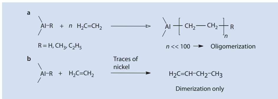
Fig. 11.2 (a) Ziegler's "Aufbaureaktion" (Chain extension reaction). (b) The nickel effect
