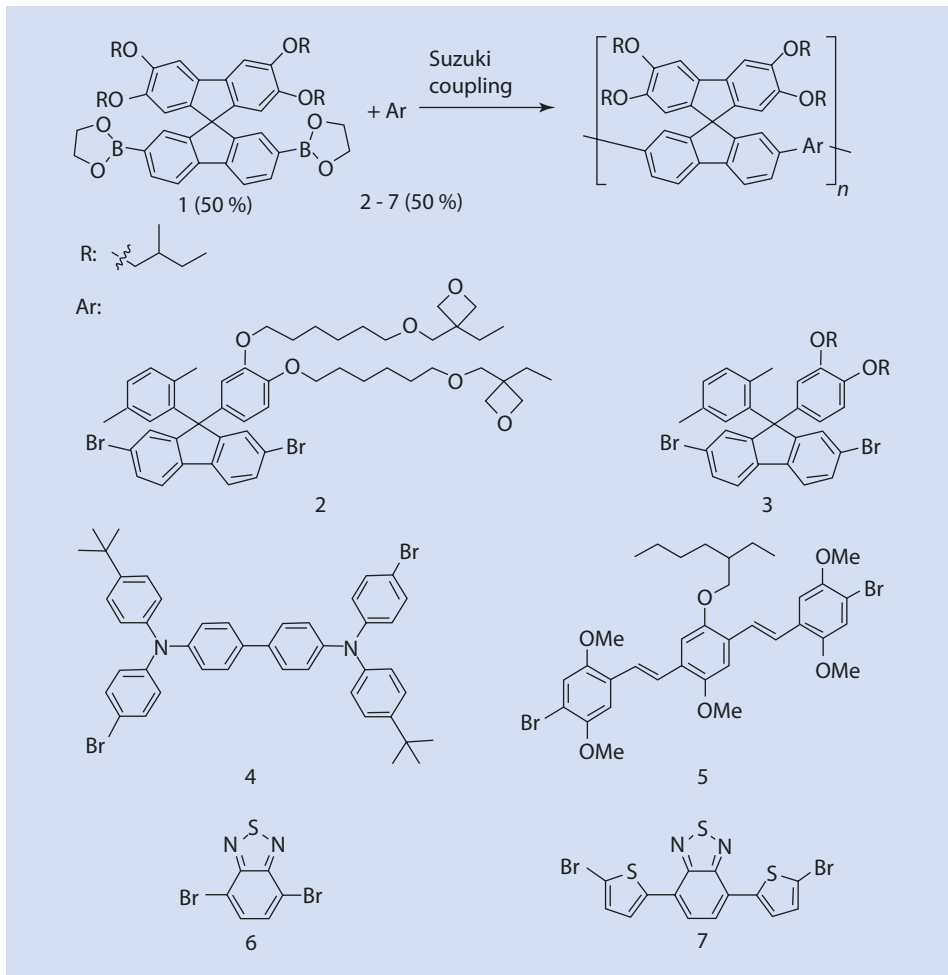
Fig. 22.15 Synthesis of blue, green, and red luminescent polymers by Suzuki-coupling
