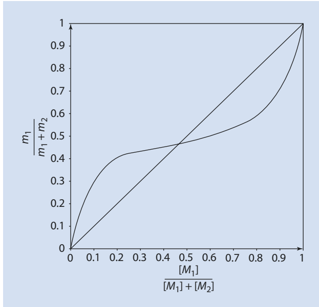
■ Fig. 13.3 Instantaneous copolymer composition as a function of the initial monomer composition using the example of the copolymerization of styrene ( M_1 ) and acrylonitrile ( M_2 )
