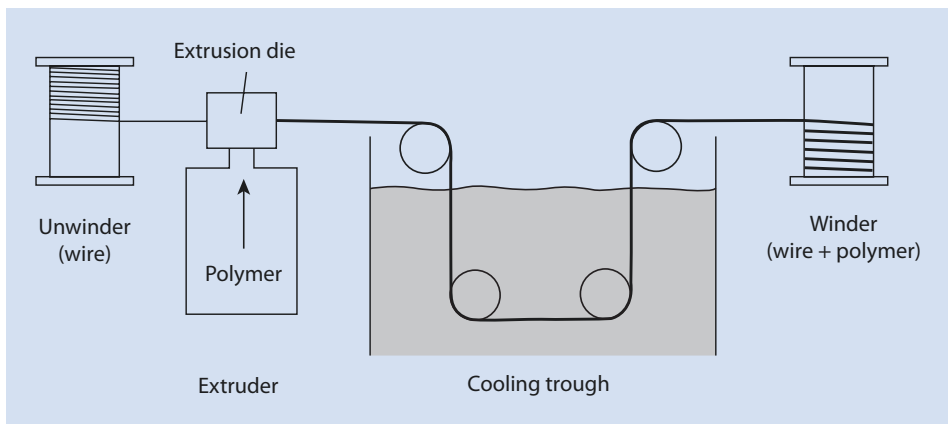
■ Fig. 17.5 Simplified diagram of a wire sheathing machine
