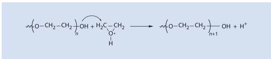
Fig. 12.11 CROP: activated-monomer mechanism
