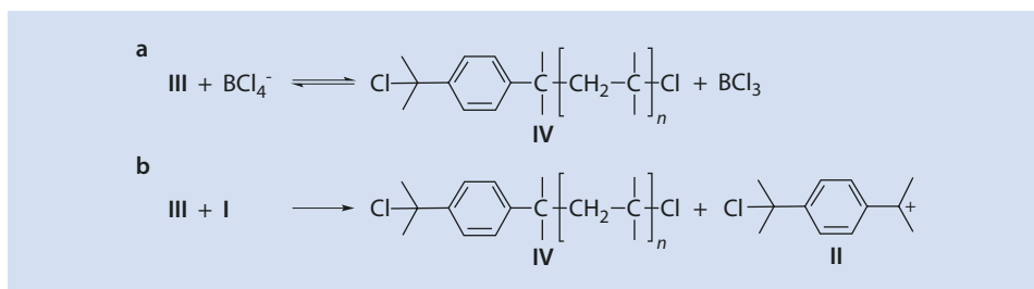
Fig. 10.36 INIFER-mechanism: termination of propagation by: (a) anion splitting or (b) the initiator
