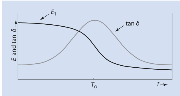
Fig. 4.9 Graph of the storage modulus and the loss factor as a function of temperature
