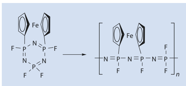
■ Fig. 12.52 Synthesis of a polyphosphazene with a ferrocene side chain
