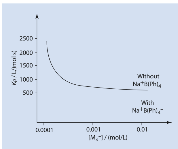
■ Fig. 10.77 Typical plot of the propagation rate constants experimentally determined for a polymerization involving both free ions and ion pairs (e.g., sodium naphthalene styrene in THF)
