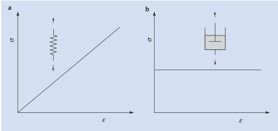
■ Fig. 6.8 \sigma = f(\dot{\epsilon}) : (a) for an elastic material (storage of energy); (b) for a viscous fluid (dissipation of energy)
