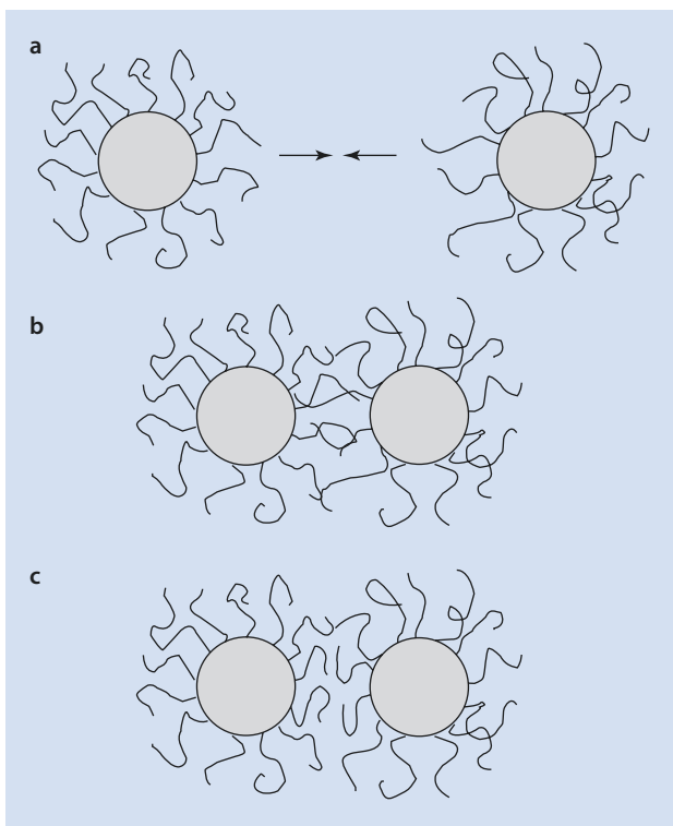
Fig. 19.5 Scheme showing the processes occurring when two sterically stabilized colloid particles approach each other. (a) Starting condition. (b) Approach involving an entanglement of the polymer chains. (c) Approach involving a compression of the polymer chains
