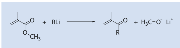
■ Fig. 10.72 Nucleophilic substitution of the \text{OCH}_3 -group of the monomer by R
