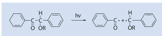
■ Fig. 9.7 Photochemical decomposition of benzoin ether
