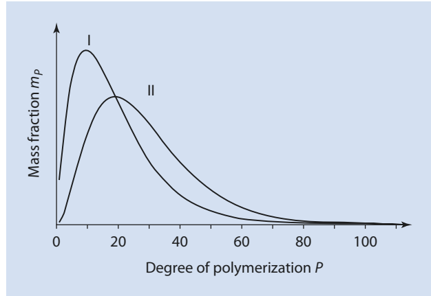
Fig. 9.24 Mass distribution function for \nu = 10 , calculated from (9.63) and (9.69). I/Termination by Disproportionation, II/Termination by Combination
