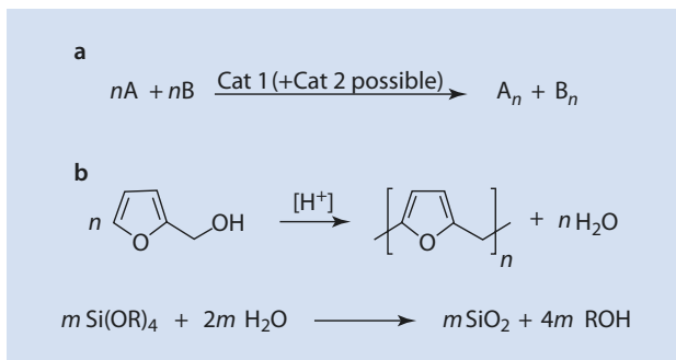
■ Fig. 22.1 Simultaneous polymerization. (a) Schematically. (b) Example: polymerization of furfuryl alcohol and tetraalkoxysilane
