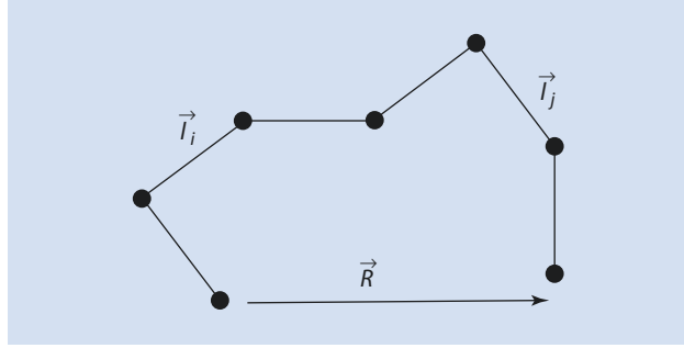
■ Fig. 2.2 The Gaussian chain model with different repeating units (e.g., \vec{l}_i and \vec{l}_j ), which are described by vectors according to their spatial position. \vec{R} is a measure of the distance between the chain ends
