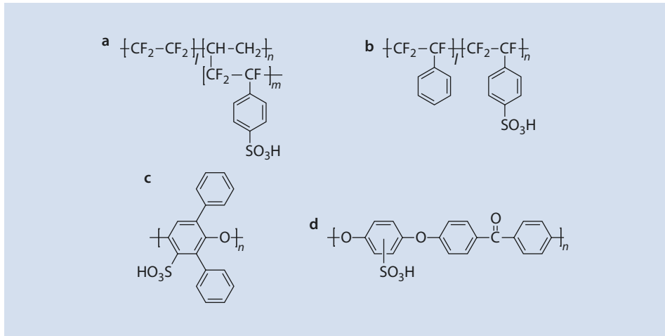
■ Fig. 22.21 Selected examples of proton conductors. (a) Scherer (1990). (b, c) Ballard Power Systems. (d) Maier and Meier-Haack (2008)
