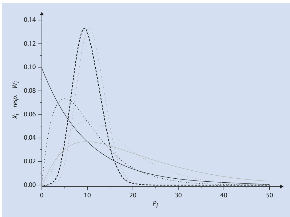
■ Fig. 10.88 Distribution functions with P_n = 10 . Dashed line: Poisson-distribution, full line: Schulz-Zimm distribution with \zeta = 1 , dotted line: Schulz-Zimm distribution with \zeta = 2 . (black: mole/number fraction distributions x_i , gray: weight fraction distributions w_i )
