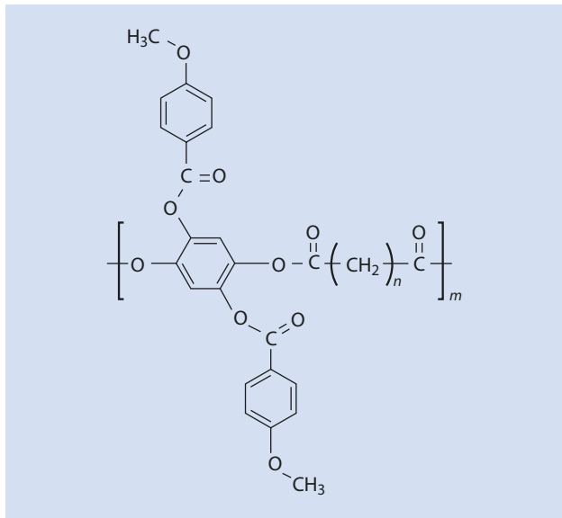
■ Fig. 20.17 Lateral arrangement of a mesogen group in the main chain. n = 10, 12, 14, 20
