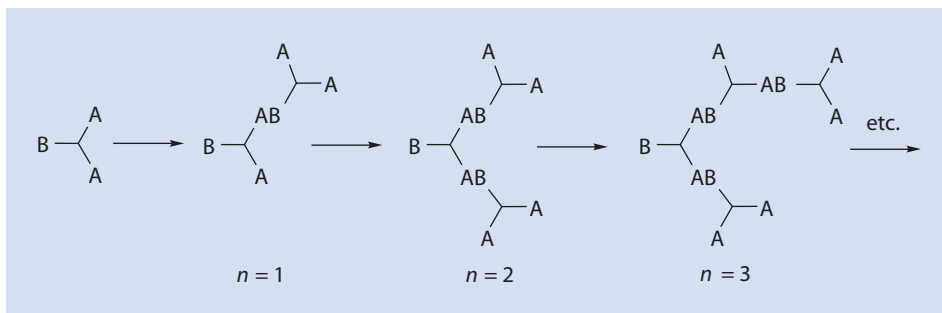
■ Fig. 8.16 Formation of hyperbranched polymers from A_2B -monomers
