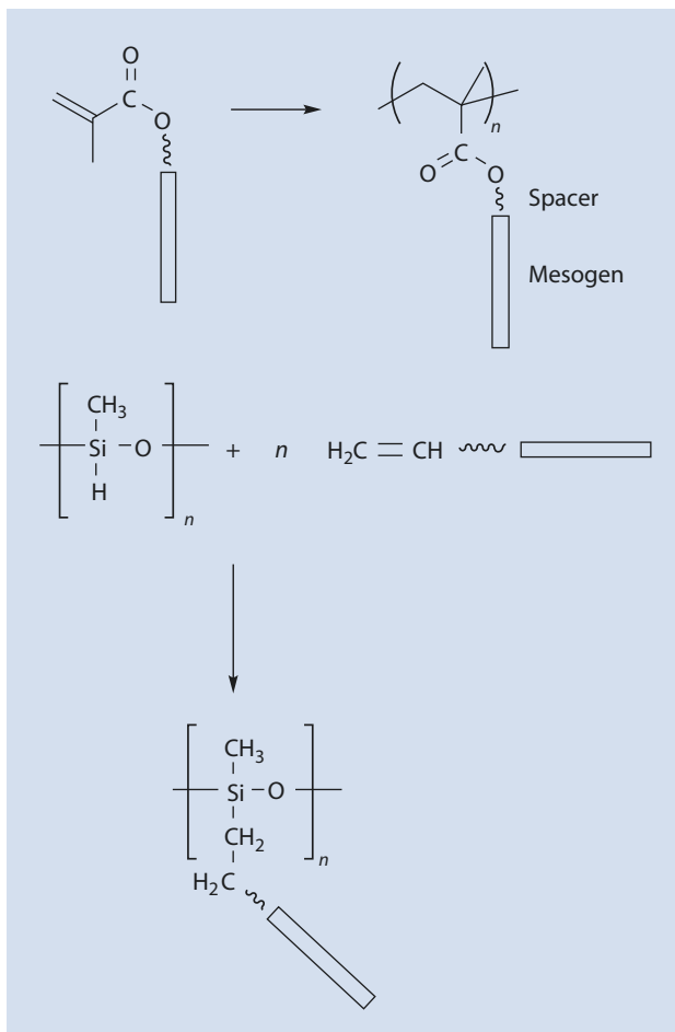
Fig. 20.19 Synthetic route to SCLP
