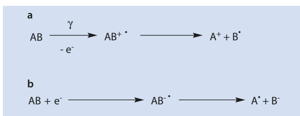
■ Fig. 9.8 Creation of radicals with high energy radiation. (a) \gamma -Radiation. (b) \beta -Radiation
