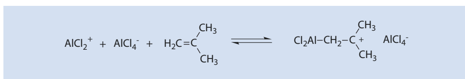
■ Fig. 10.13 Initiation of the polymerization of isobutene with \text{AlCl}_3 via self-dissociation (in the absence of water)
