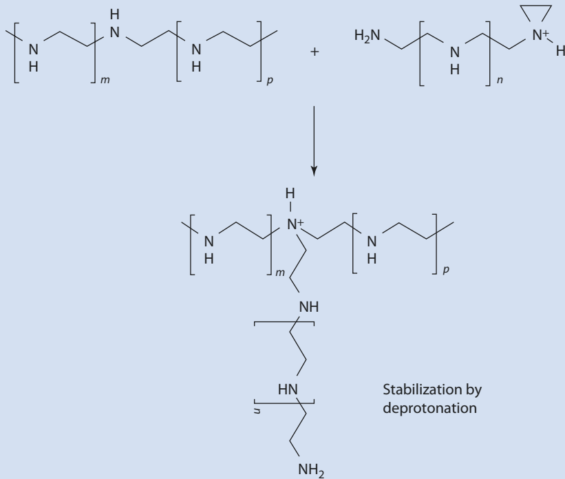
■ Fig. 19.3 Polymerization of ethylene imine to polyethylene imine
